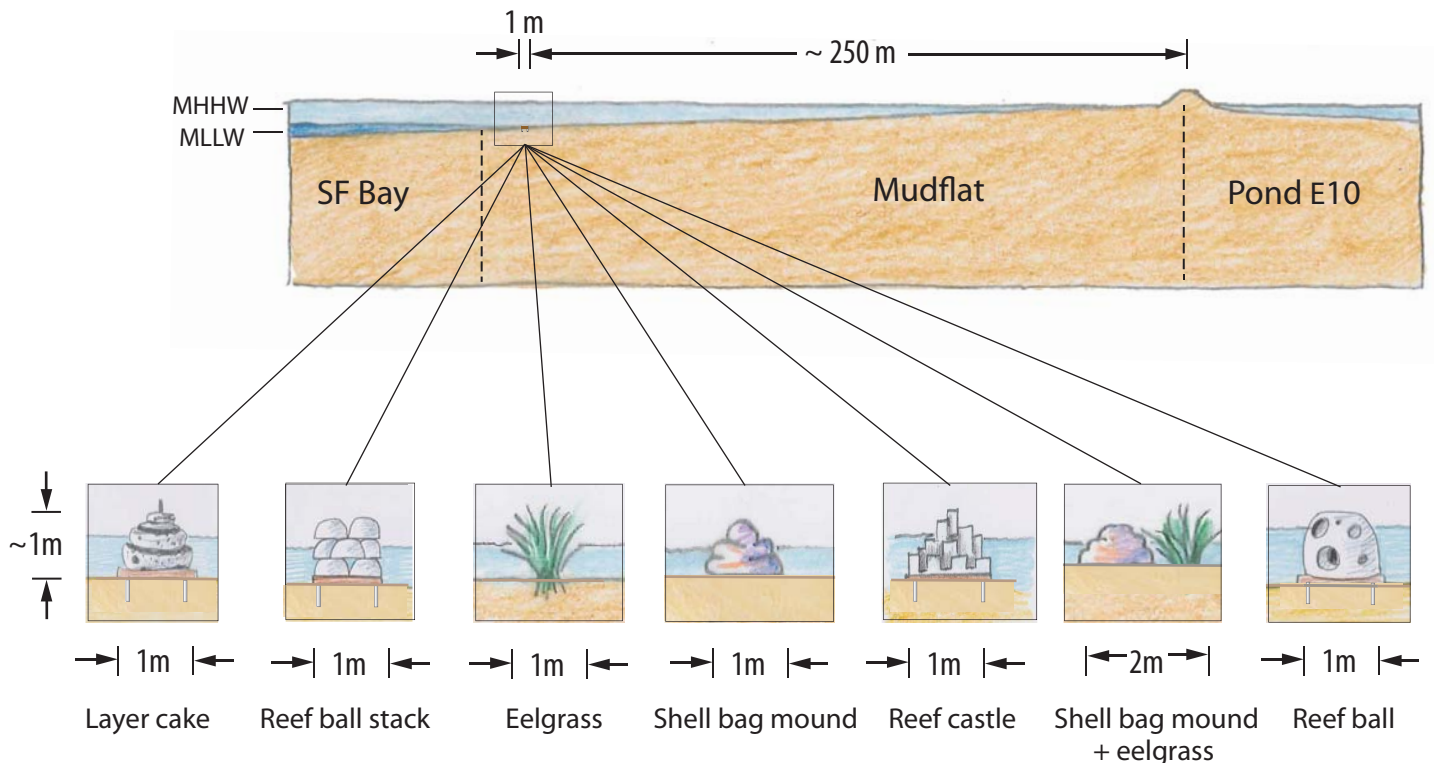
Substrate Elements at Hayward Shoreline North Cross Section
